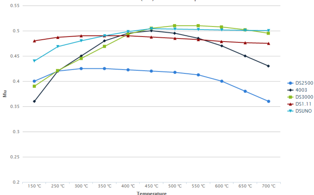
Friction Coefficient ( \mu ) Versus Temperature
